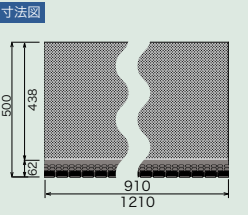
PX-5723 NEW (910mm 巾) PX-5724 NEW (1210mm 巾)
